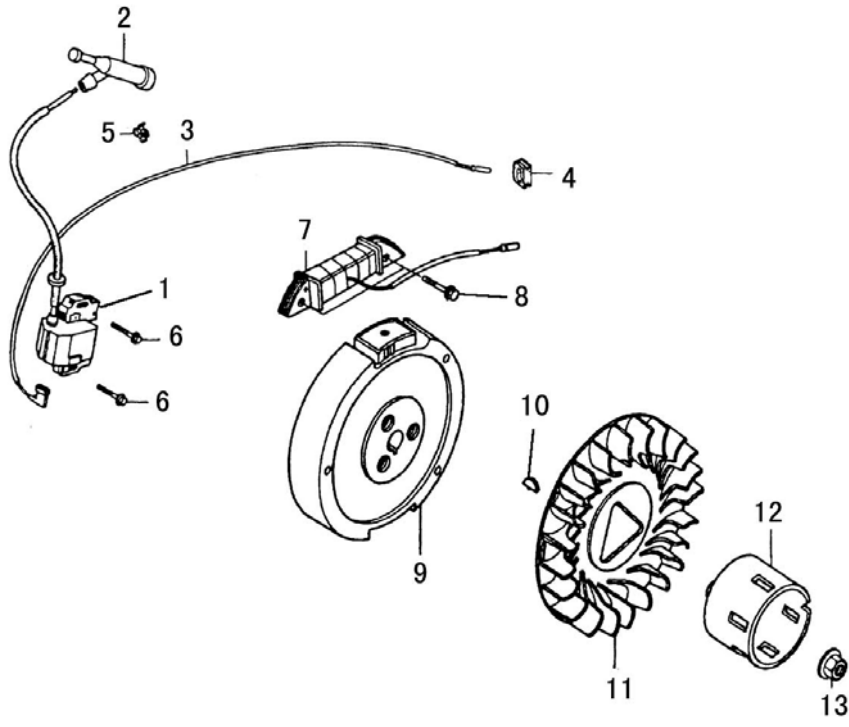
FIG.J FLYWHEEL
